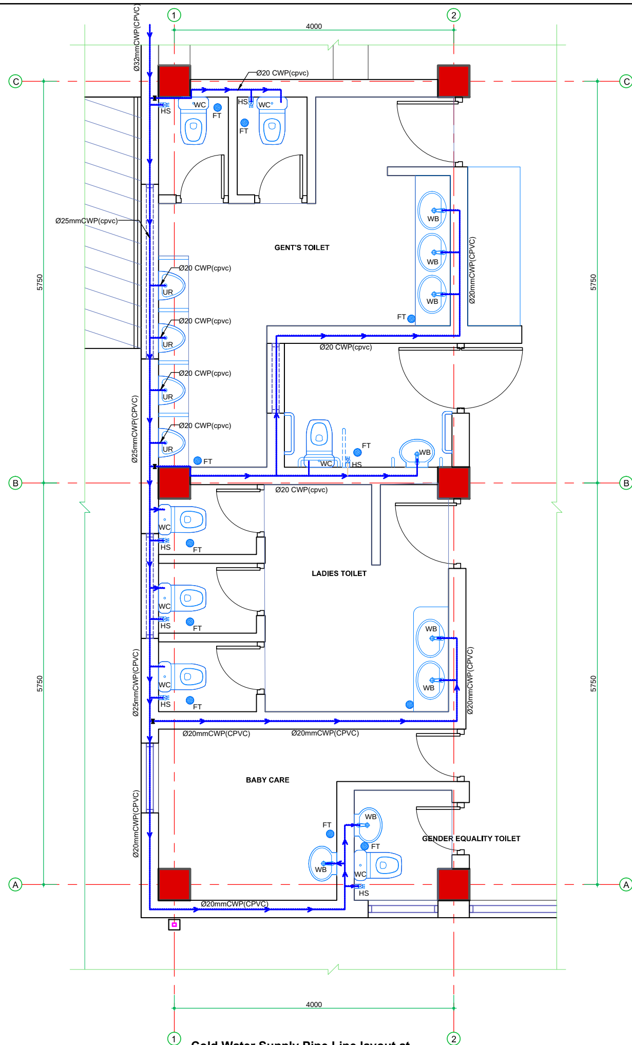
Cold Water Supply Pipe Line layout at (Ground Floor) (Scale:-1:50)
